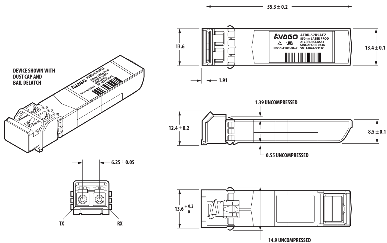
Figure 5. Module drawing.
