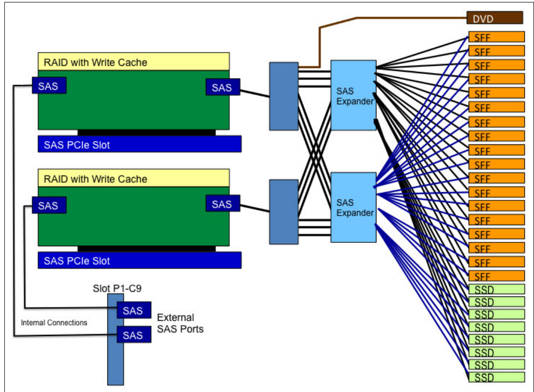
Figure 2-20 Internal topology overview for the #EJ0P DASD backplane
