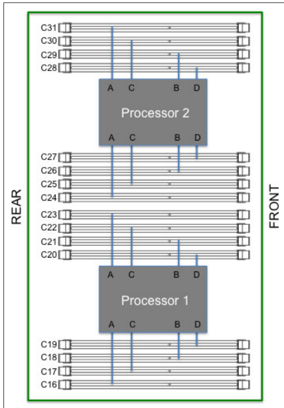
Figure 2-10 Memory DIMM topology for the Power S814 and Power S824
