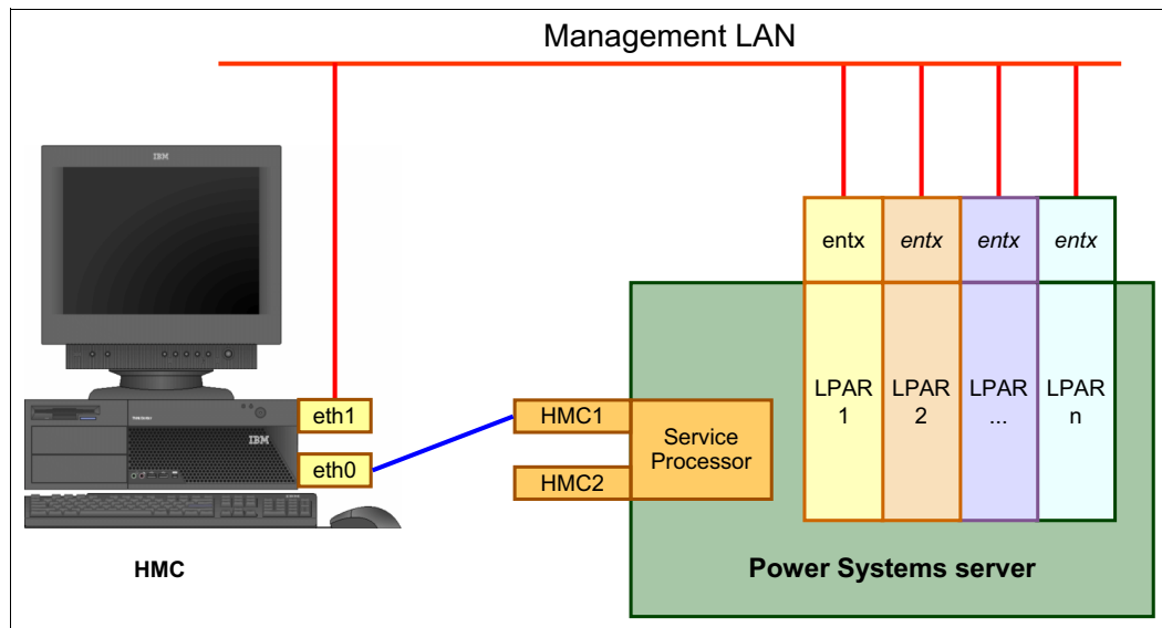
Figure 2-25 Network connections from the HMC to service processor and LPARs
