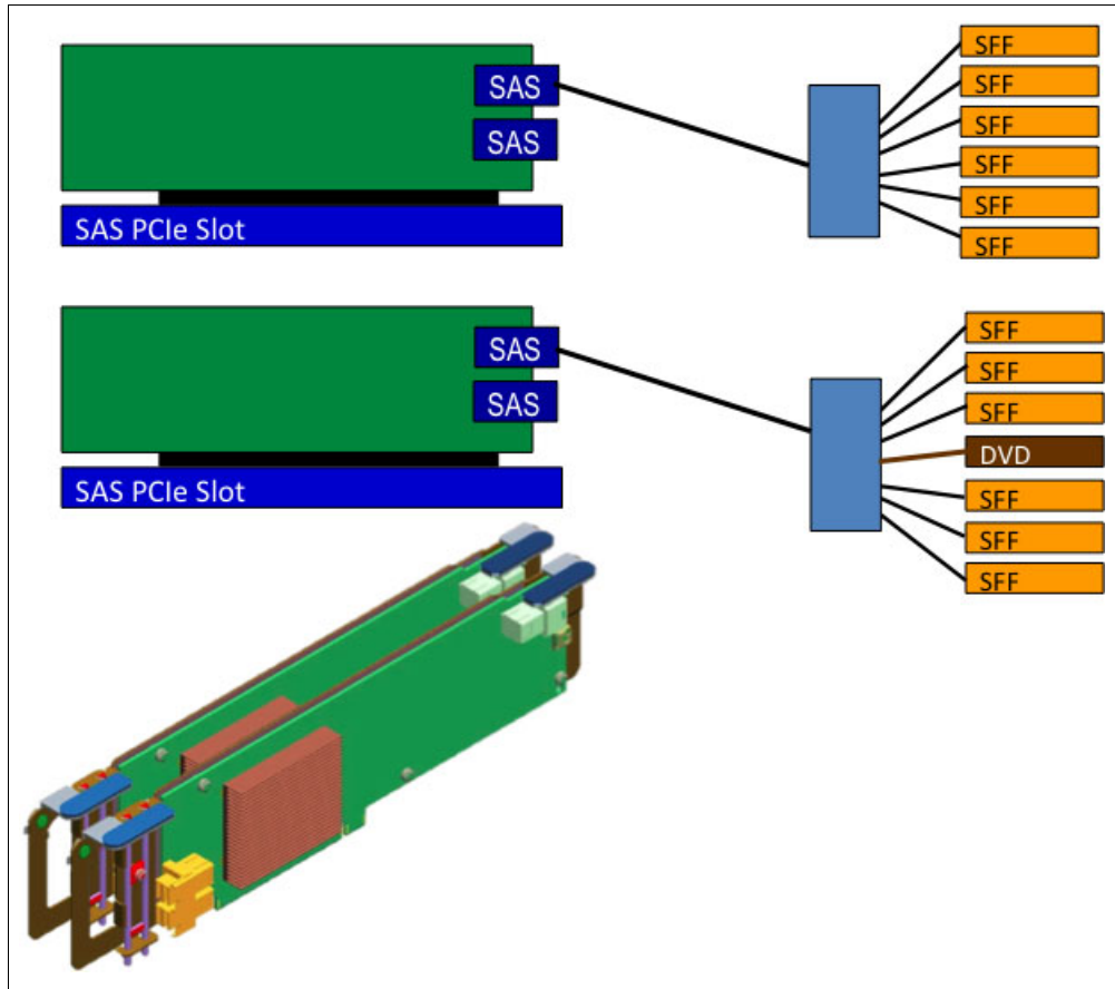
Figure 2-19 Internal topology overview for the #EJ0N DASD backplane with the #EJ0S split backplane feature
