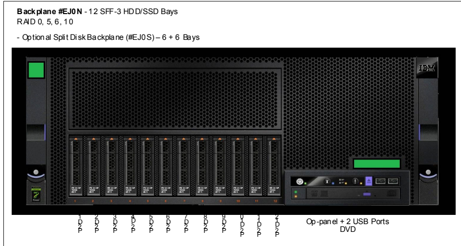
Figure 2-16 Server front view with #EJ0N backplane option
