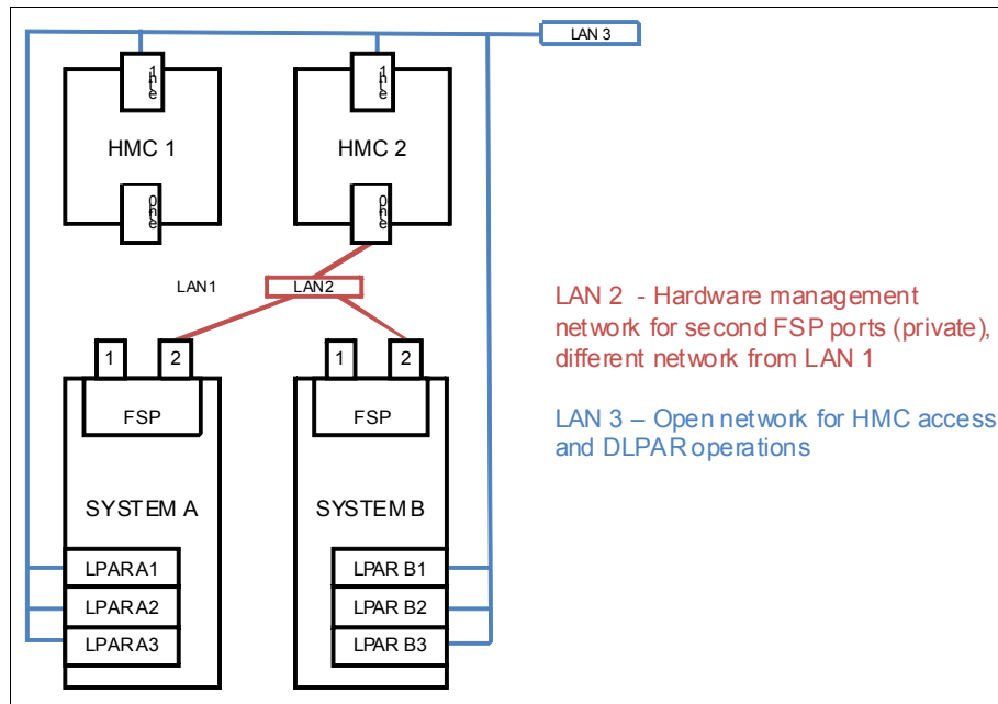
Figure 2-26 Highly available HMC networking example
