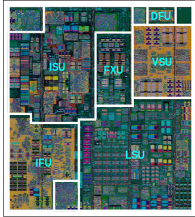
Figure 2-5 POWER8 processor core
