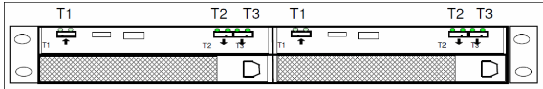
Figure 2-24 EXP24S SFF Gen2-bay drawer rear connectors
