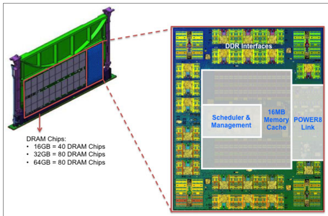
Figure 2-9 A short CDIMM on a tall CDIMM slot diagram
