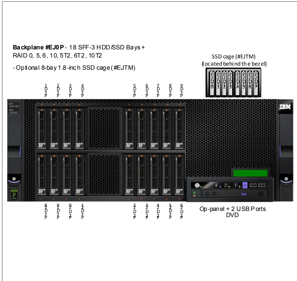
Figure 2-17 Server front view with #EJ0P backplane option
