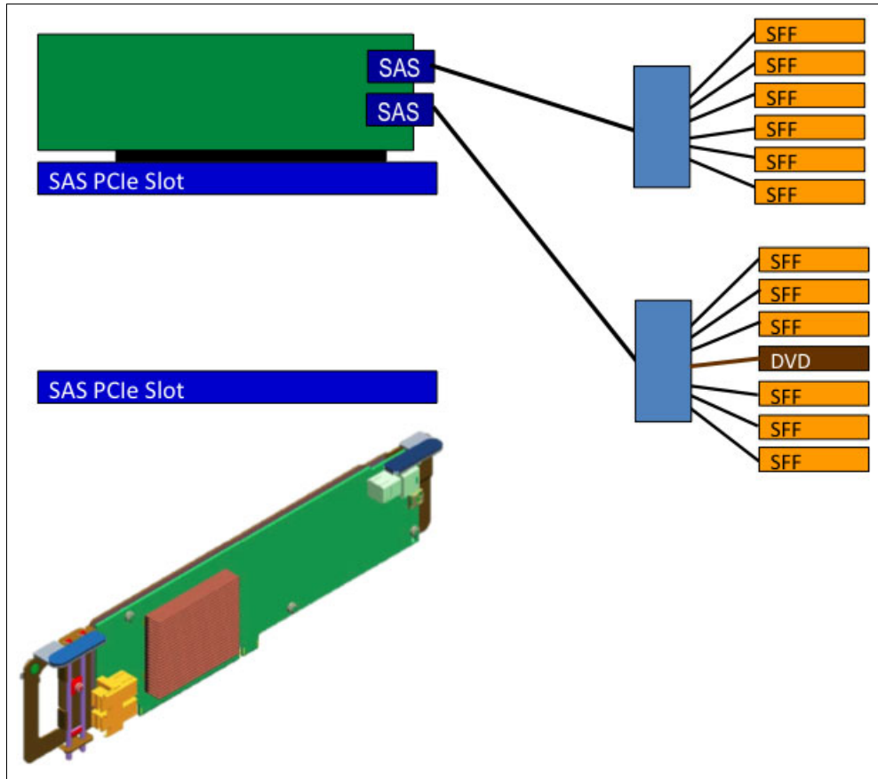
Figure 2-18 Internal topology overview for the #EJ0N DASD backplane
