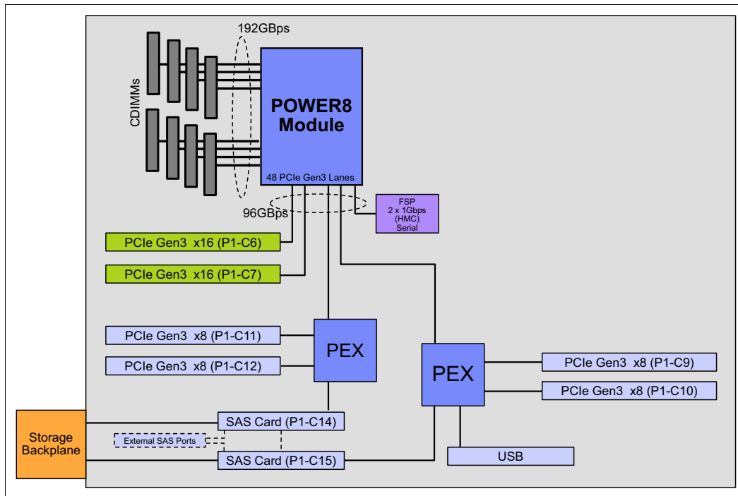
Figure 2-1 IBM Power S814 logical system diagram
