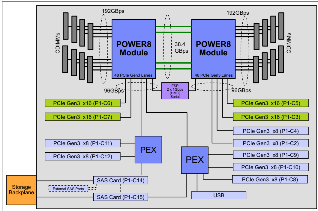
Figure 2-2 IBM Power S824 logical system diagram
